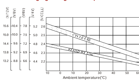
Relationship between charging voltage and temperature
